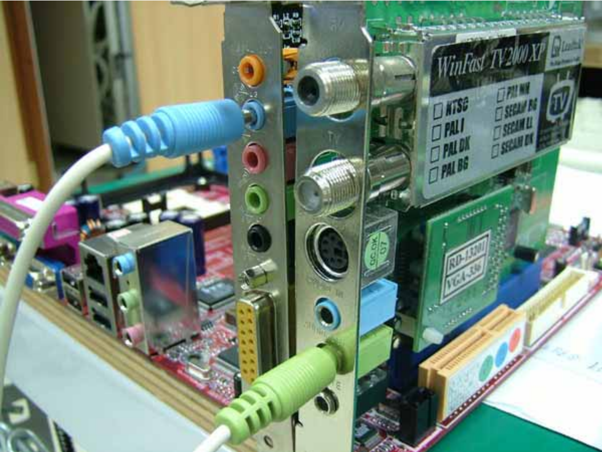
1-2 : Connect from Audio out of TV2000 XP Deluxe to sound card Line in .
